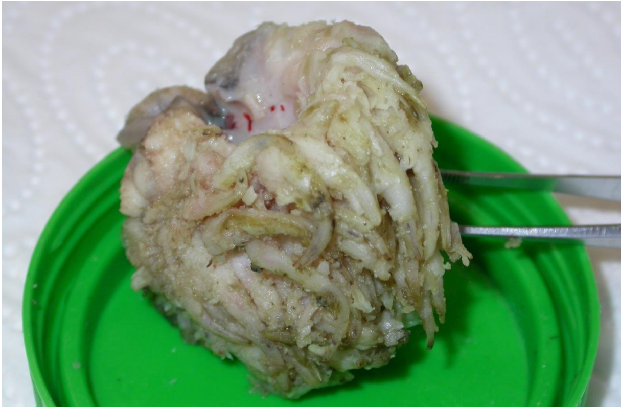
Abb. 5: Warzenmaterial Rind
