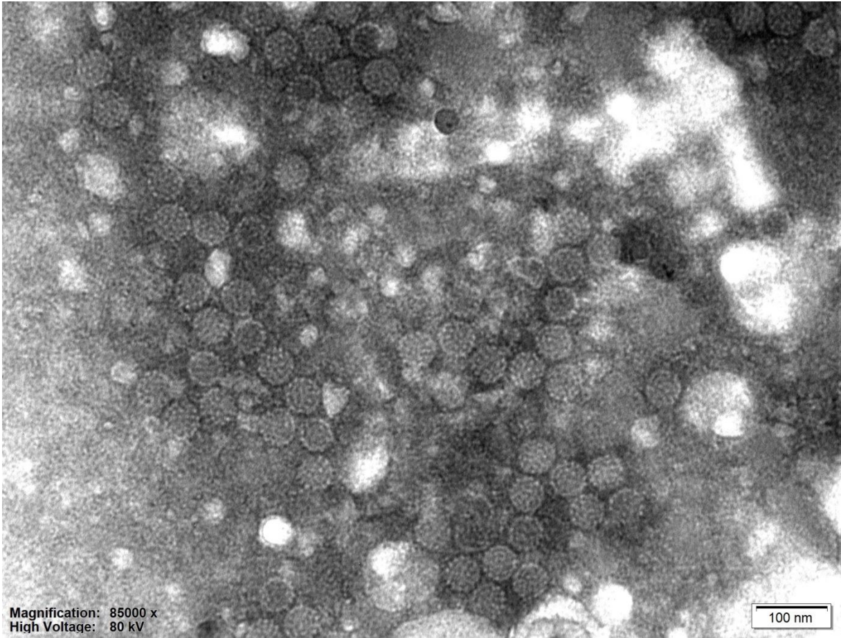
Abb. 5: Warzenmaterial Rind
